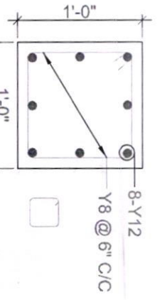
CS OF COLUMN "C3" (1'-0" x 1'-0")
