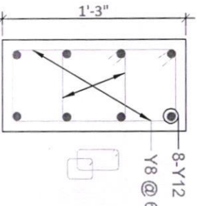
CS OF COLUMN "C1" (0'-9" x 1'-3")
