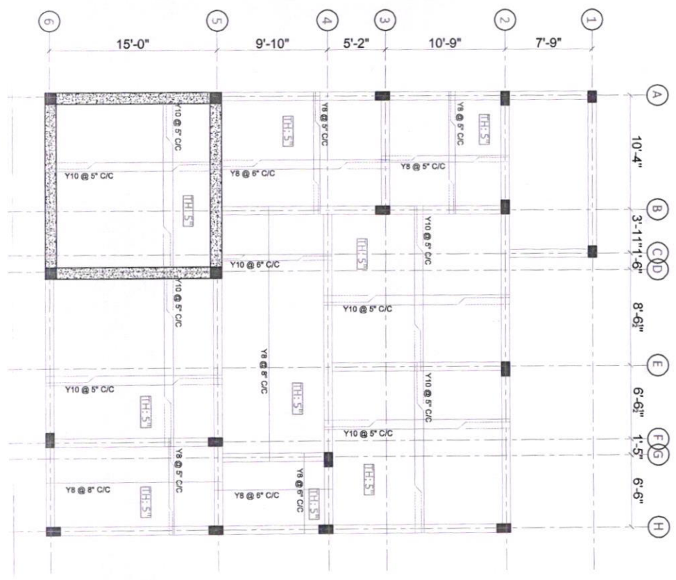
GROUND FLOOR ROOF SLAB LAYOUT
