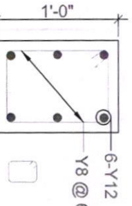
CS OF COLUMN "C2" (0'-9" x 1'-0")
